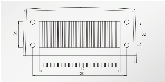
KEA 24 W90 S Cut-out for cable entry
