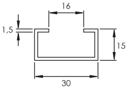
C-rail dimensions (mm)
