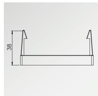
Blank plate BPK-SNAP, see page 344
