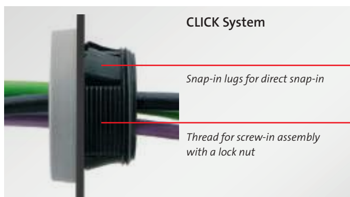
Mounting type 1: Snap into the cut-out For wall thickness 1 – 2.5 mm
