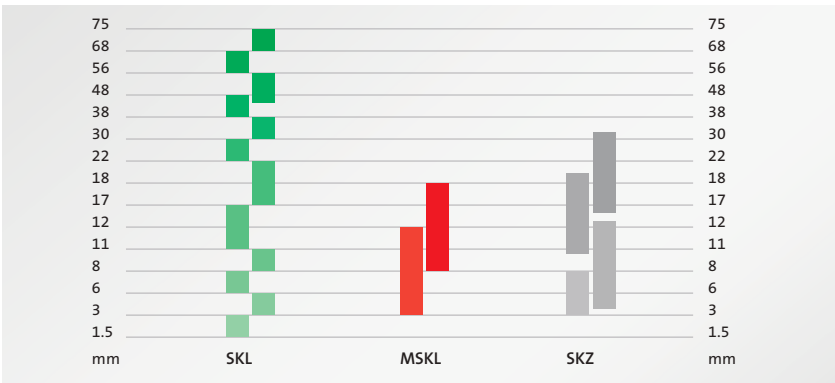
SKL | MSKL | SKZ clamping ranges
