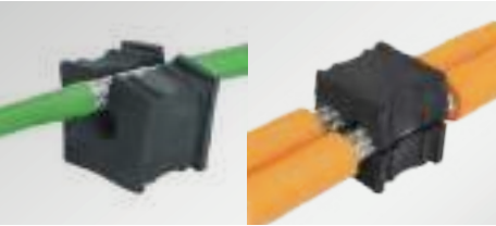
Split EMC grommets small, single and multi for cables with and without connectors for cable diameters 2 to 16 mm EMC-KT 296
