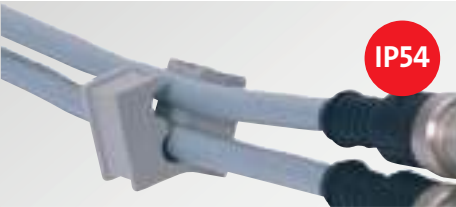
Split cable grommets, multi and special IP54 protection for cable diameters 3 to 7 mm QT multi 120
