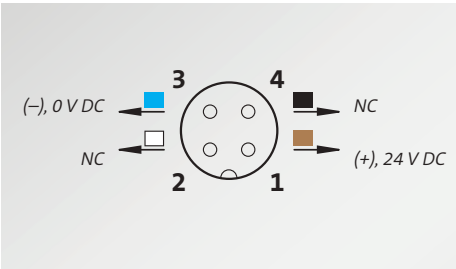
M12 connector female (SC versions)
