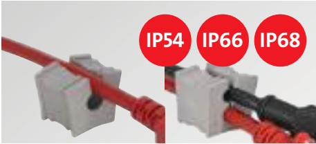
KT cable grommets split, for cables with and without connectors for cable diameters 1 – 35 mm 78, 79
